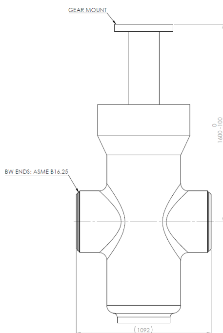
Pic 1 – distance between C.L to gear mount
